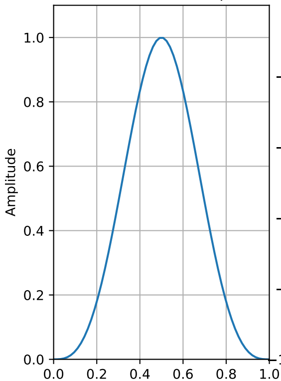
Bohman Window (64 points)
