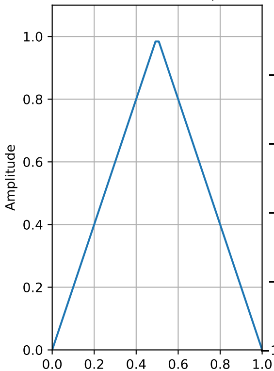
Bartlett Window (64 points)
