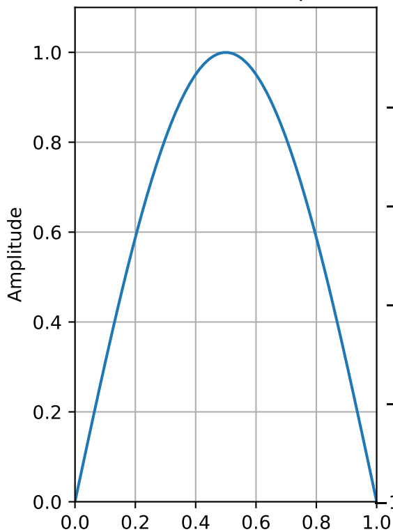
Cosine Window (64 points)
