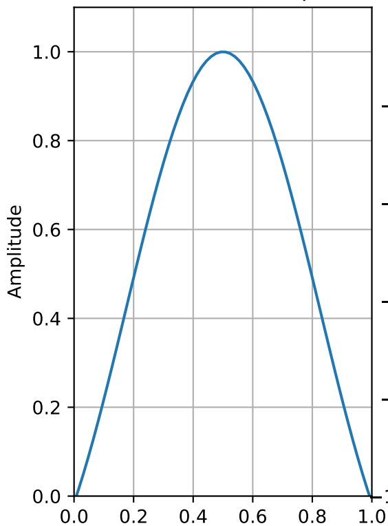
Lanczos Window (64 points)
