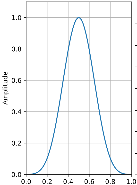
Blackman_harris Window (64 points)
