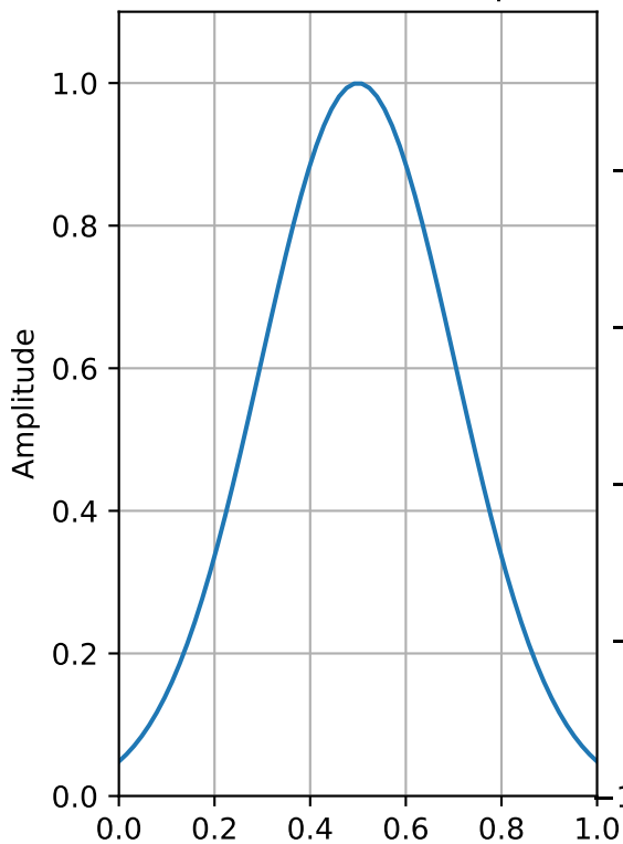
Gaussian Window (64 points)
