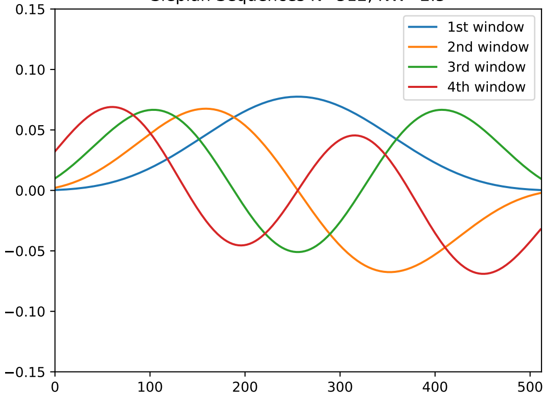
Slepian Sequences N=512 , NW=2.5
