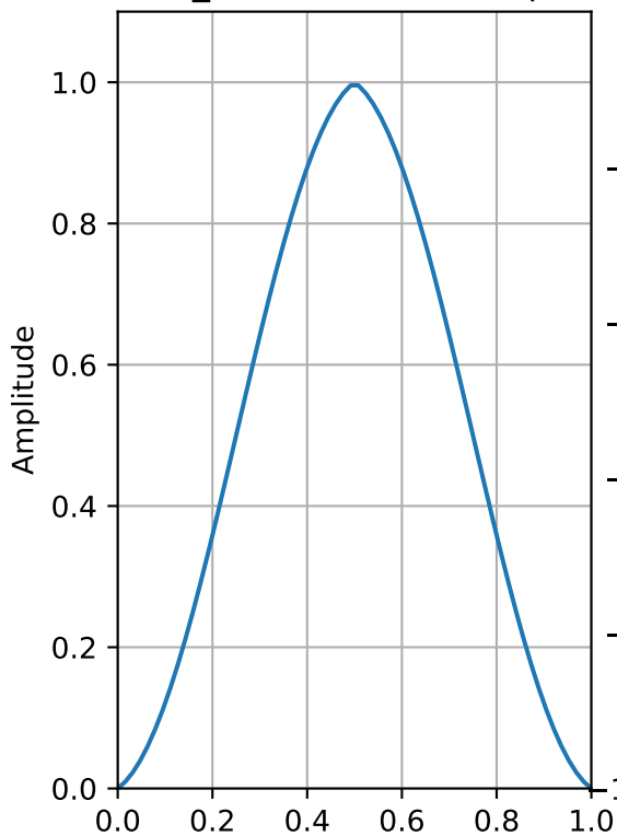
Bartlett_hann Window (64 points)
