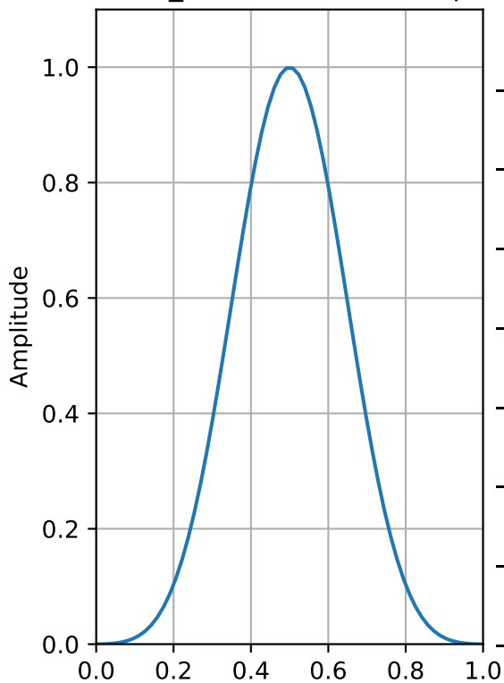
Blackman_harris Window (64 points)
