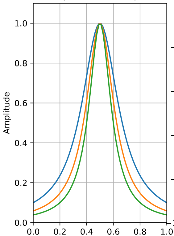
Cauchy Window (64 points)
